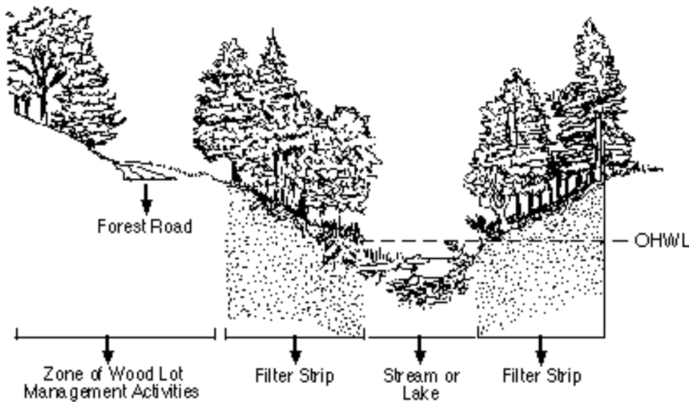
Figure 1: Areas where filter strips are needed.
