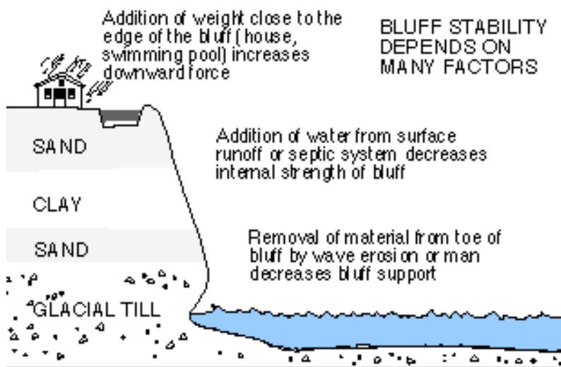
Figure 1: Factors that can make bluffs unstable.
