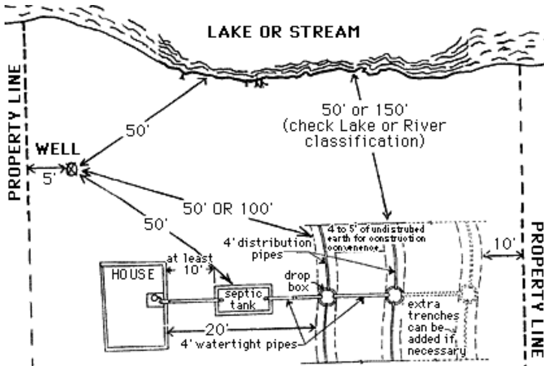
Figure 1: Sewage treatment system with minimal separation distances.
